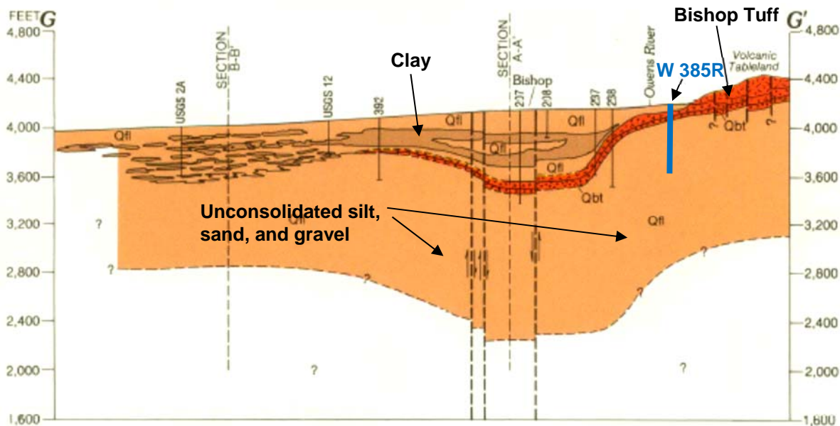
Figure 5. Hollett's Geologic Section G-G' Showing the Location of W385R
