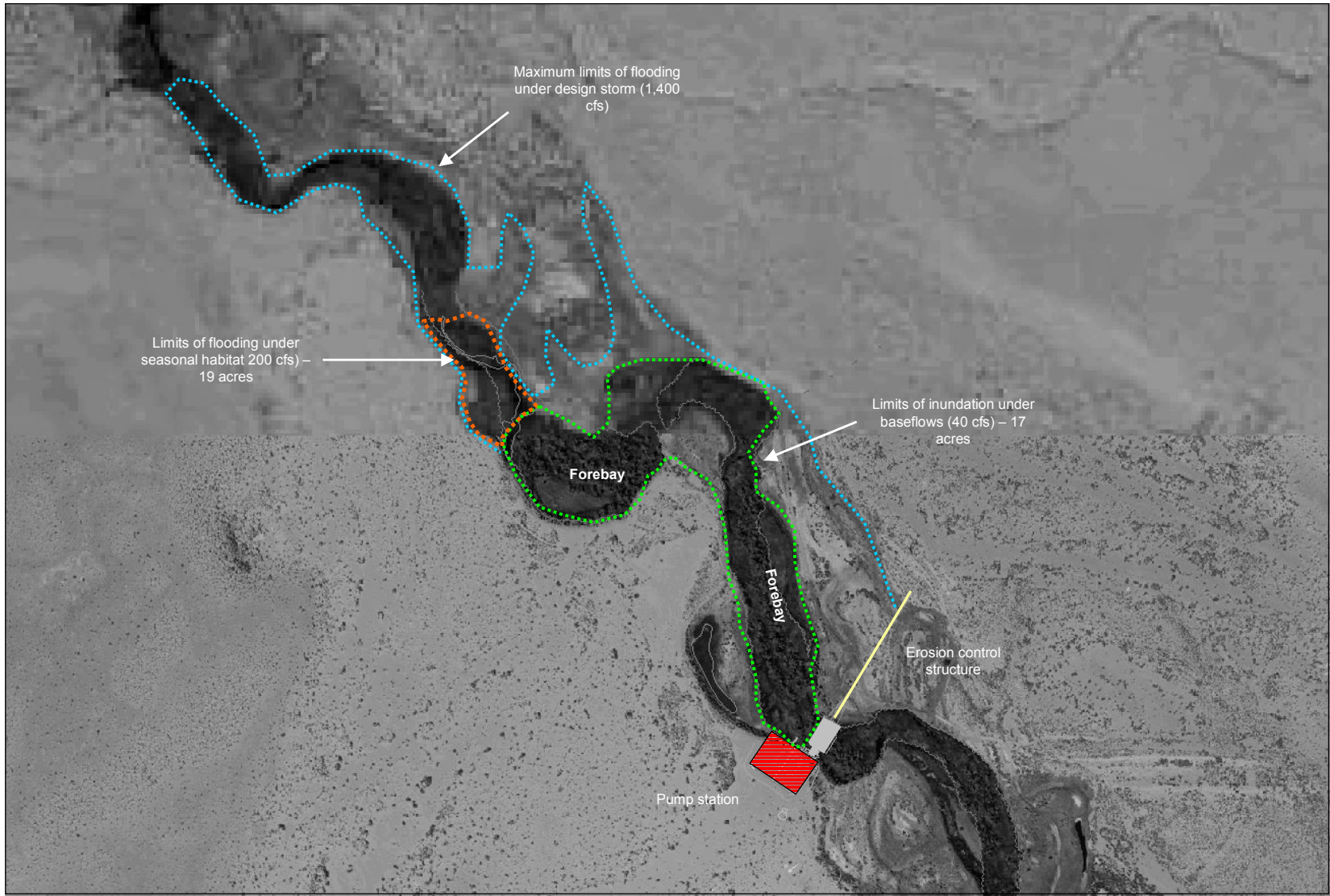
Figure 2-14. Limits of Inundation above the Pump Station
