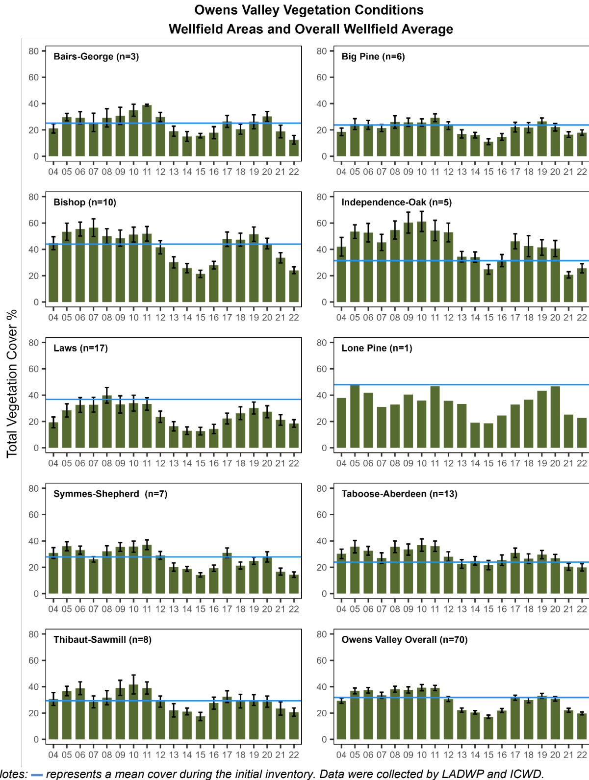
Figure 2.25. Owens Valley Vegetation Condition for Wellfields
